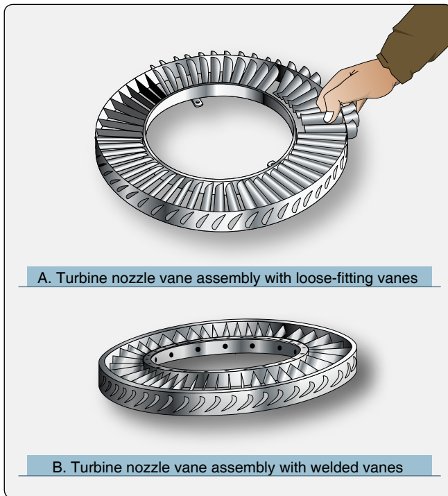
Figure 1-63. Typical turbine nozzle vane assemblies.
