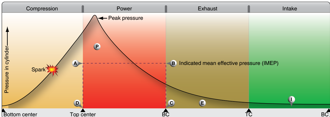
Figure 1-39. Compression ratio.
